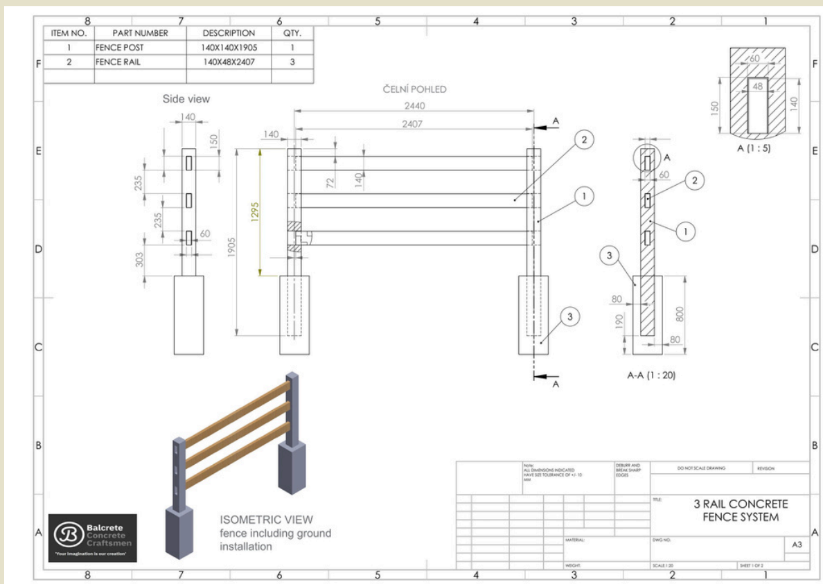
3 RAIL TECHNICAL DRAWING
