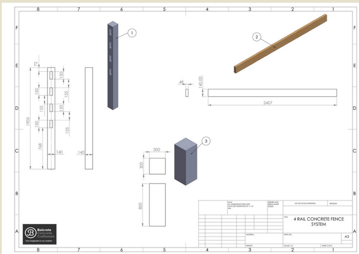
4 RAIL TECHNICAL DRAWING
