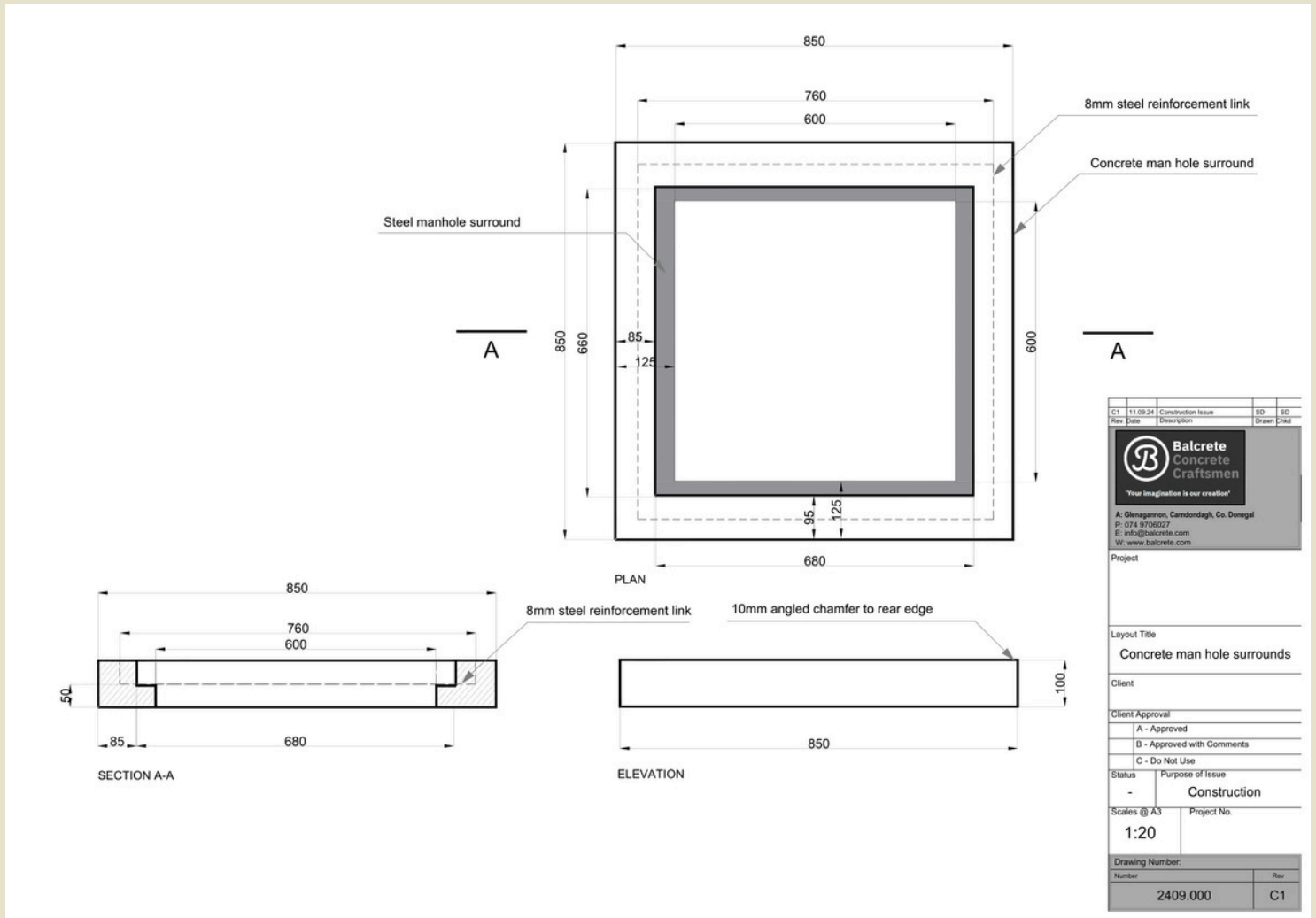
Manhole surround technical drawings
